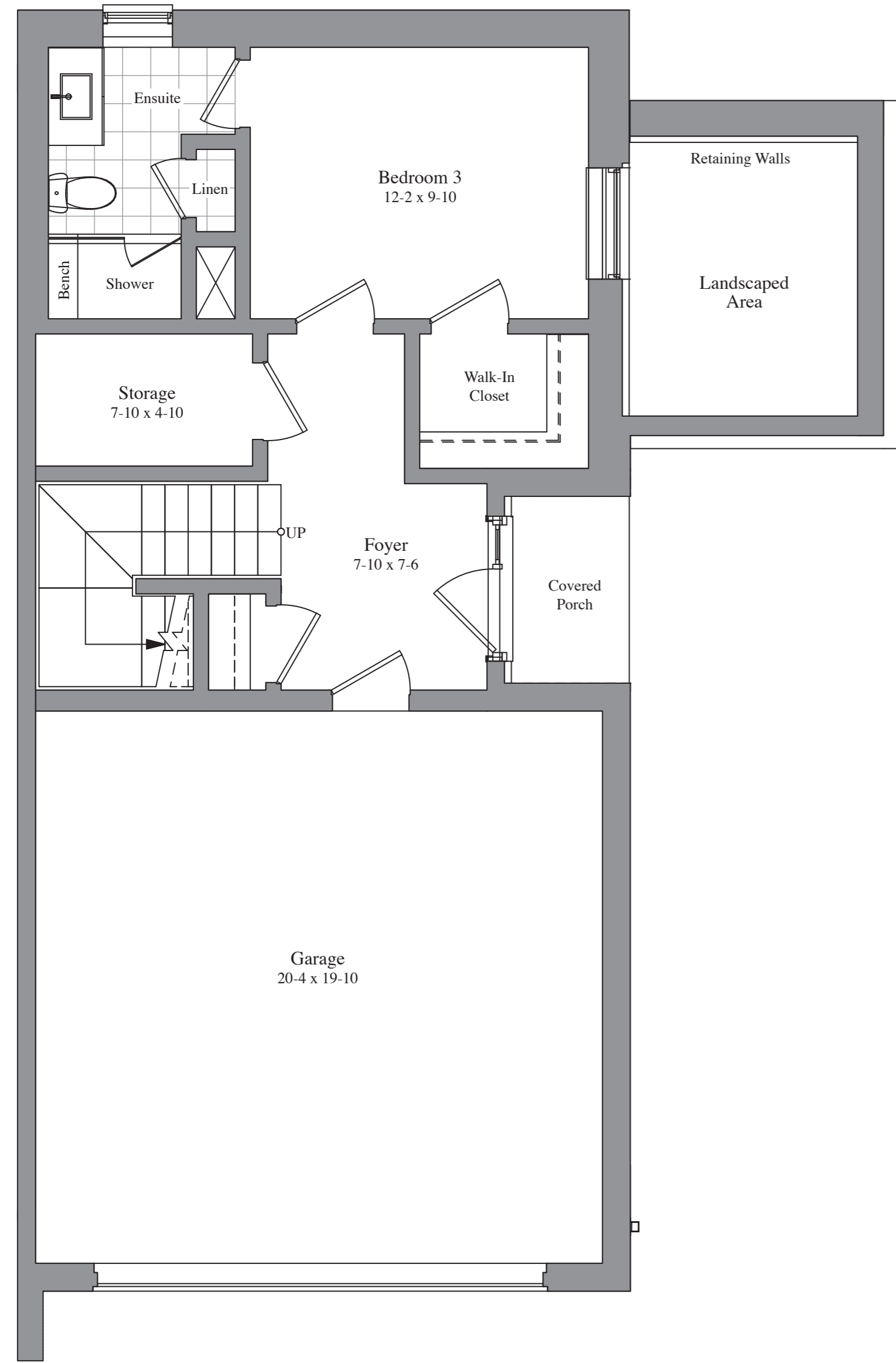
BASEMENT FLOOR PLAN ELEVATION A
