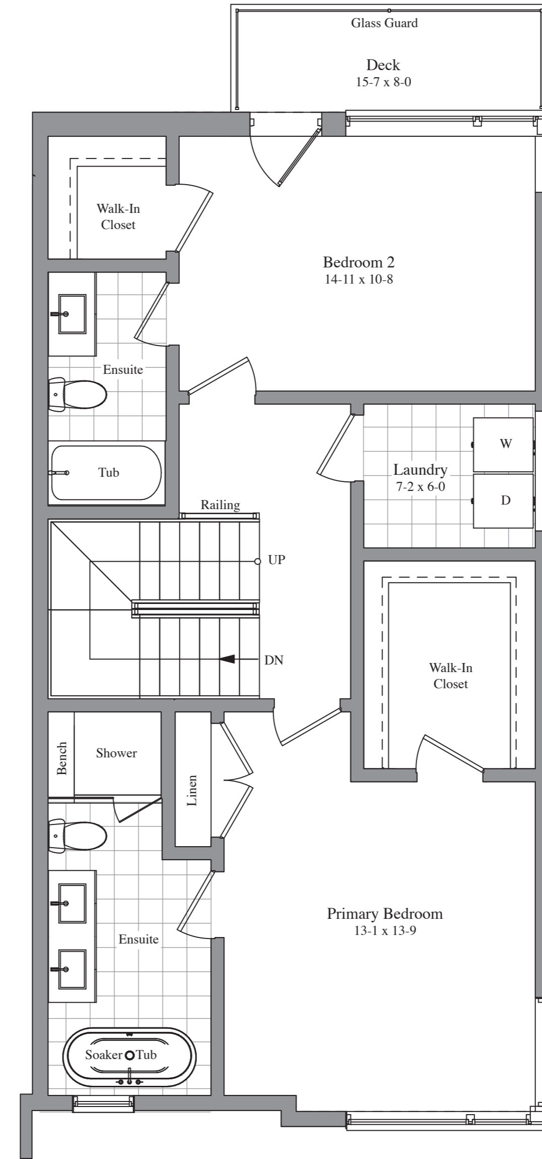
SECOND FLOOR PLAN ELEVATION A
