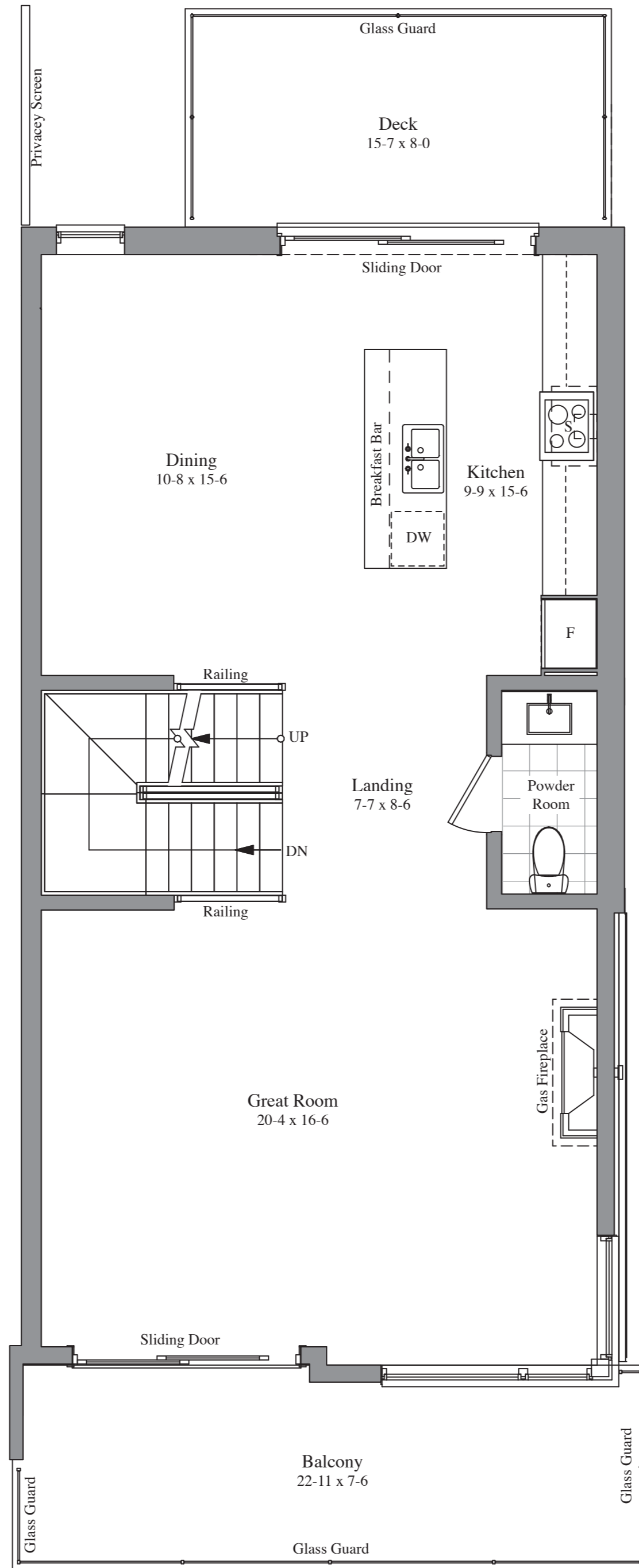
MAIN FLOOR PLAN ELEVATION A
