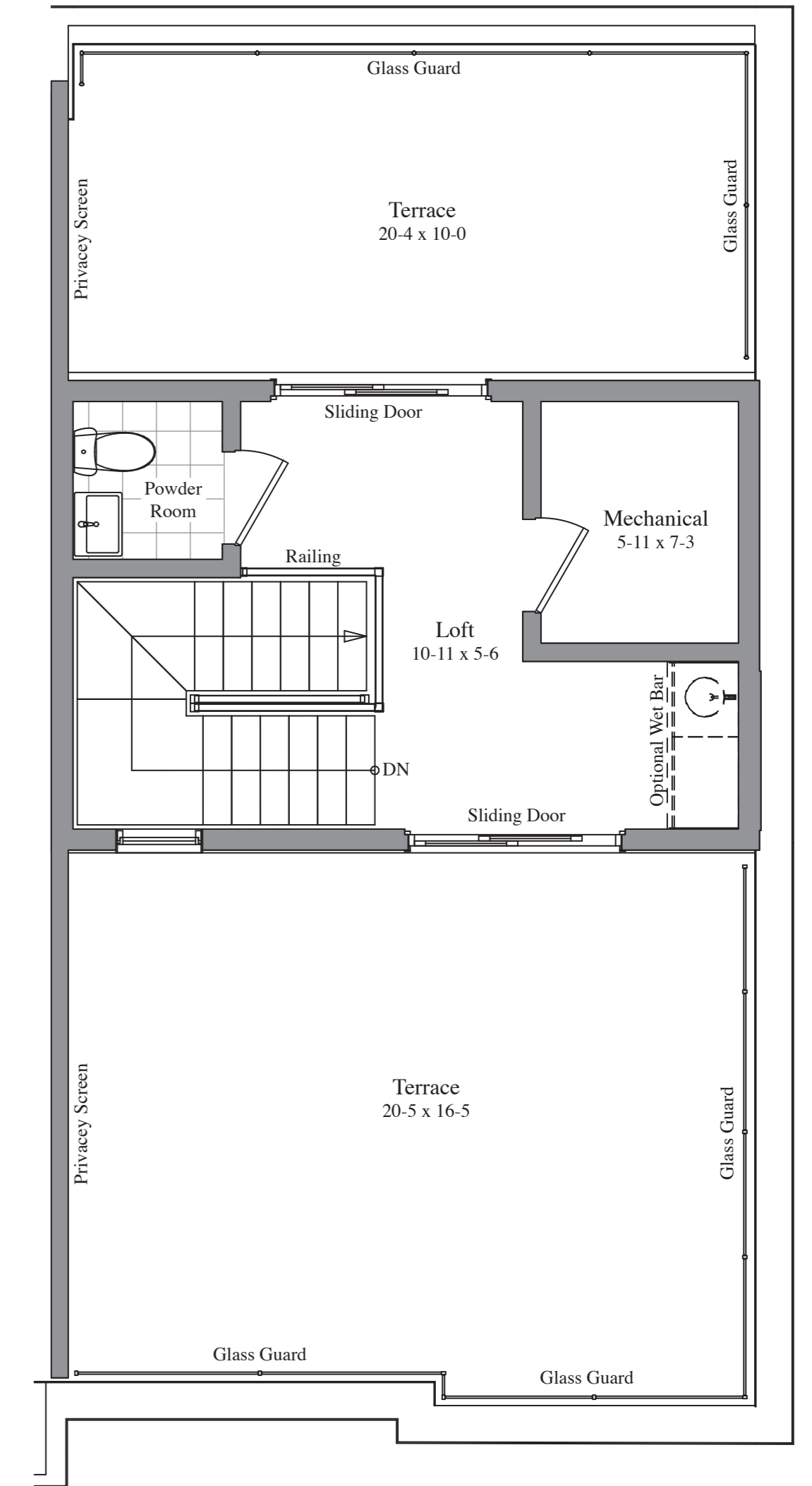
LOFT FLOOR PLAN ELEVATION A
