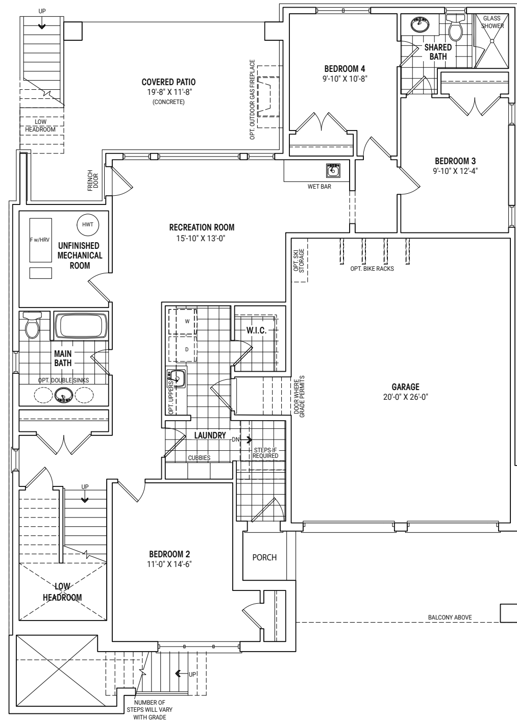
GROUND FLOOR PLAN ELEVATION C
